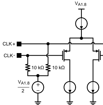
Figure 32. Equivalent Clock Receiver
