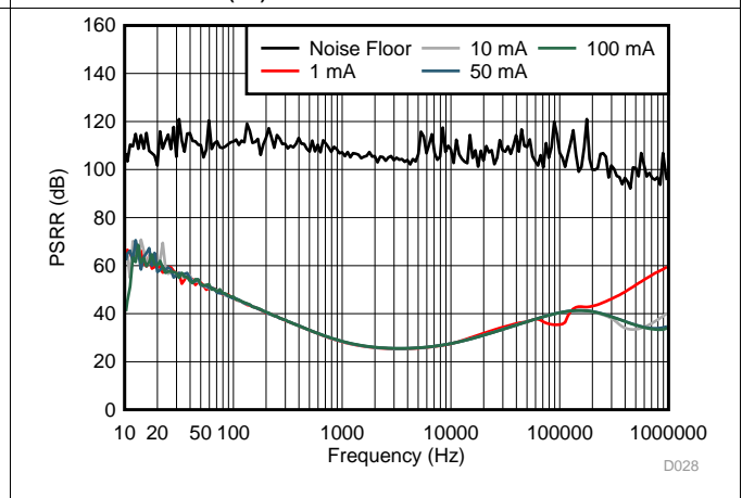
图 14. LS/LDO PSRR vs Frequency
