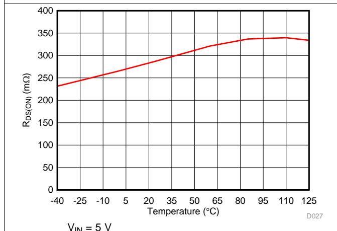
图 13. R_{DS(ON)} of Low Side MOSFET vs Temperature
