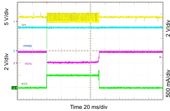
图 80. Short Circuit and Recovery for SYS
