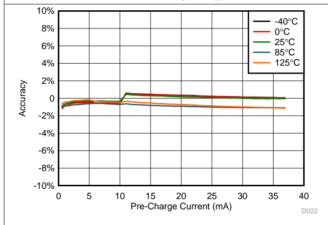
图 11. Pre-Charge Accuracy vs Pre-Charge Current
