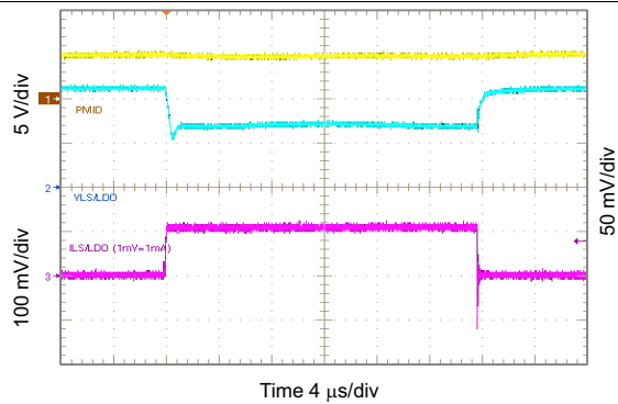
图 89. 1.2 V_{LSLDO} Load Transient, 0 to 100 mA
