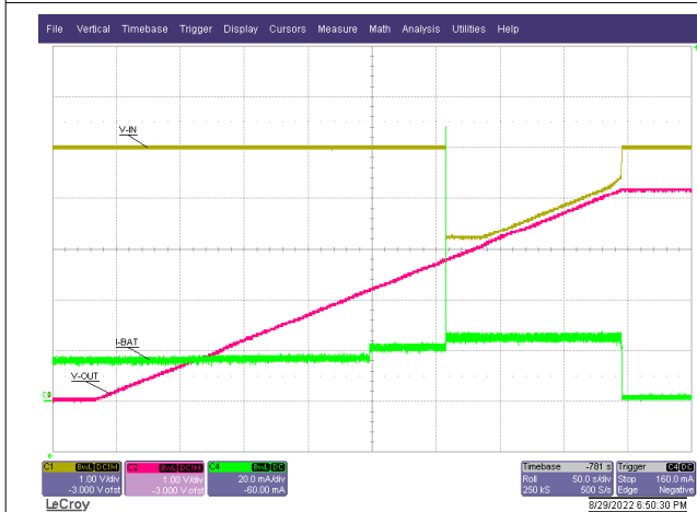
R_{ISET} = 1.5\text{ k}\Omega V_{SET} = 4.2\text{ V} Input source I_{limit} = 25\text{ mA}
