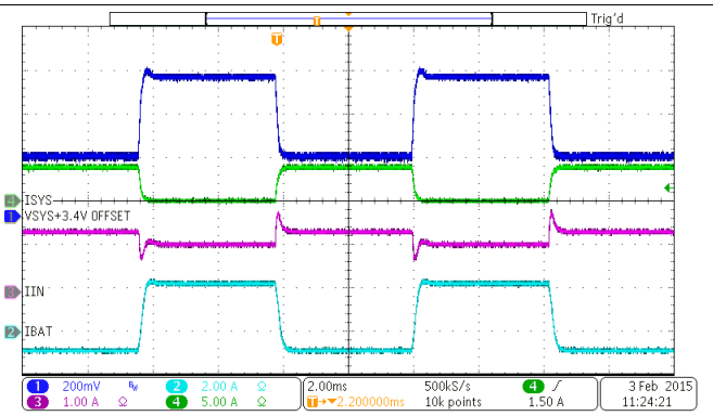
图 55. Load Transient During Supplement Mode
