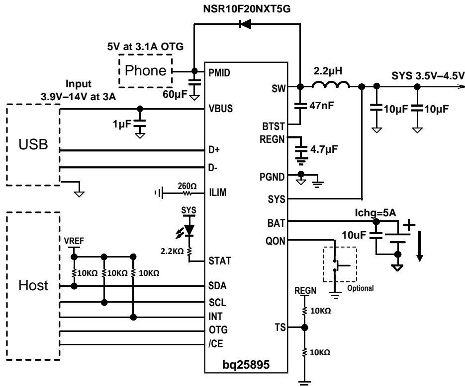
图 60. bq25895 with D+/D- Interface, 3.1 A Boost Mode Output, and no Thermistor Connections
