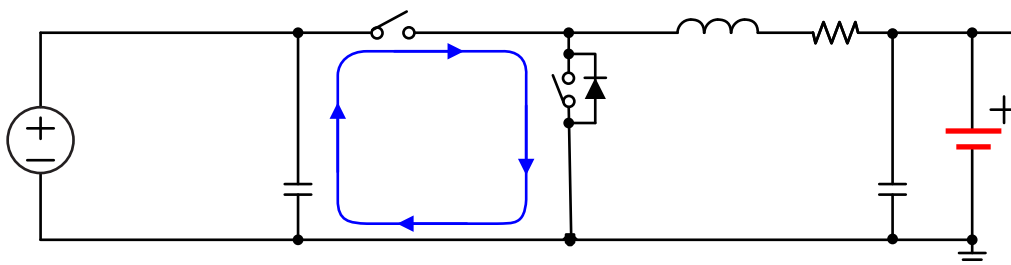
图 61. High Frequency Current Path
