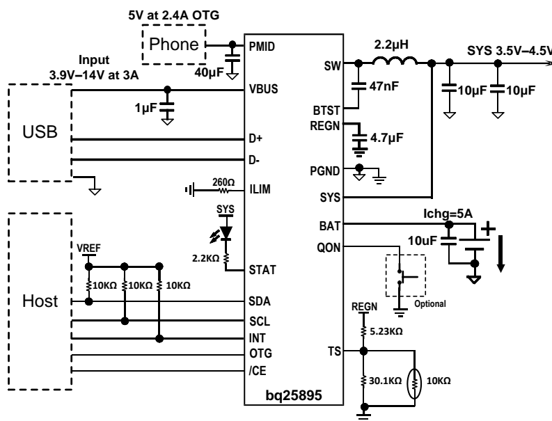
图 47. bq25895 with D+/D- Interface and 2.4 A Boost Mode Output
