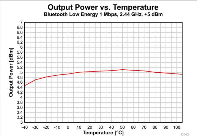
Fig 7-18. Output Power vs. Temperature (Bluetooth Low Energy 1 Mbps, 2.44 GHz, +5 dBm)
