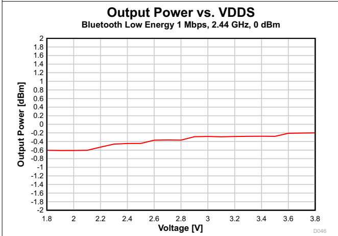
Fig 7-19. Output Power vs. Supply Voltage (VDD5) (Bluetooth Low Energy 1 Mbps, 2.44 GHz)
