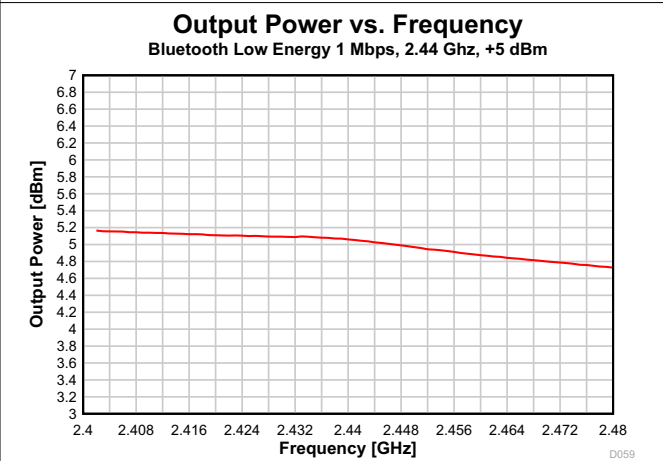
Fig 7-22. Output Power vs. Frequency (Bluetooth Low Energy 1 Mbps, 2.44 GHz, +5 dBm)
