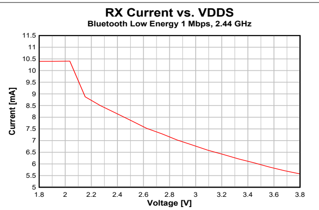
图 7-7. RX Current vs. Supply Voltage (VDD5) (Bluetooth Low Energy 1 Mbps, 2.44 GHz)
