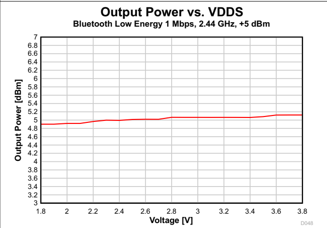
Fig 7-20. Output Power vs. Supply Voltage (VDD5) (Bluetooth Low Energy 1 Mbps, 2.44 GHz, +5 dBm)
