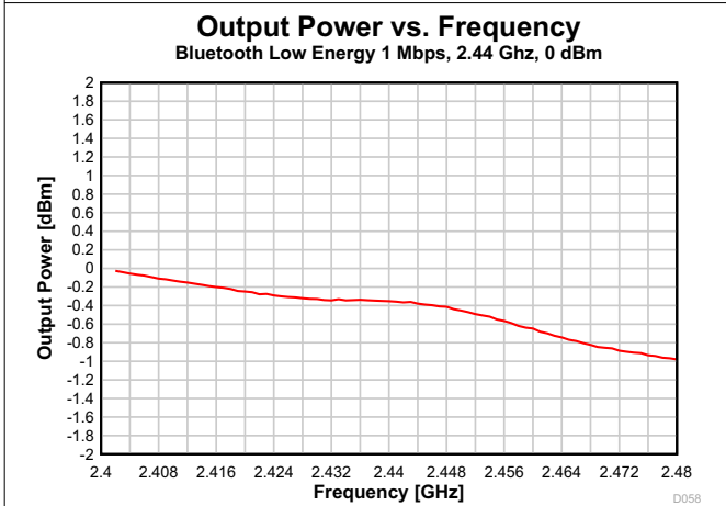
Fig 7-21. Output Power vs. Frequency (Bluetooth Low Energy 1 Mbps, 2.44 GHz)
