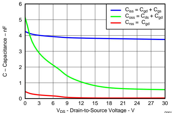
Figure 5. Capacitance
