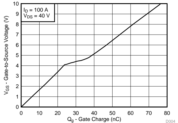
栅极电荷
