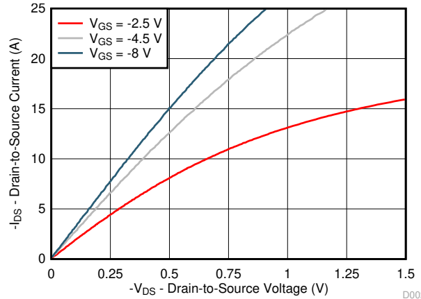
图 5-2. Saturation Characteristics
