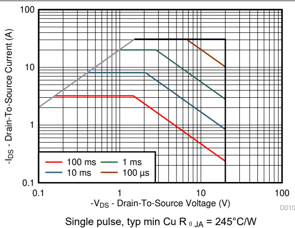
图 5-10. Maximum Safe Operating Area (SOA)
