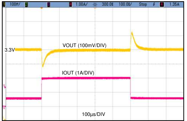
V_{OUT} = 3.3\text{ V} 400\text{ kHz} I_{LOAD} = 0.5\text{ A} - 2\text{ A} Slew Rate = 1\text{ A}/\mu\text{s}
