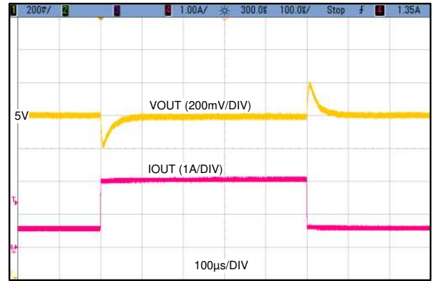
V_{OUT} = 5\text{ V} 400\text{ kHz} I_{LOAD} = 0.5\text{ A} - 2\text{ A} Slew Rate = 1\text{ A}/\mu\text{s}
