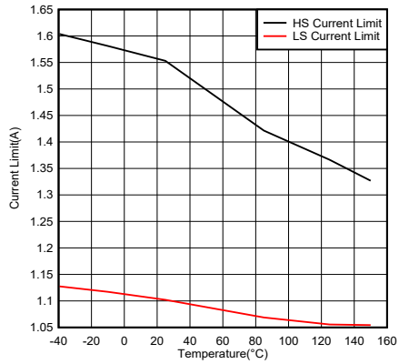
图 7-13. HS and LS Current Limit Versus Temperature
