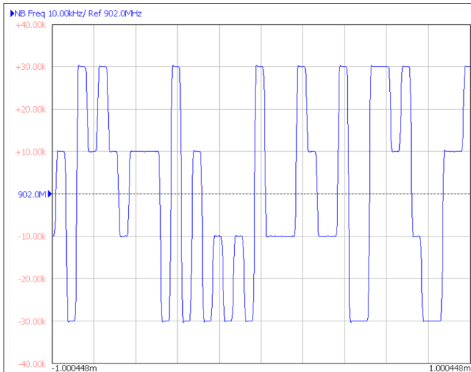
Figure 69. 4FSK Modulation
