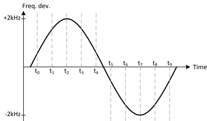
Figure 52. Over-Sampling Modulation Signal
