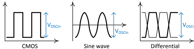
Figure 54. Input Clock Definition
