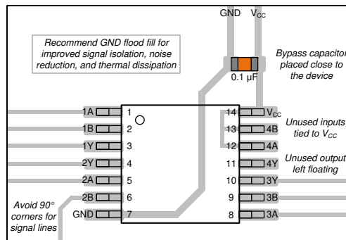
图 11. Example layout for the SN74HCS7266
