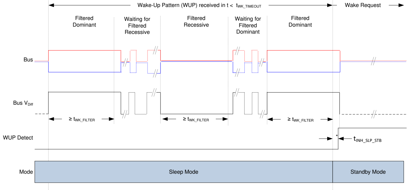
图 8-5. Wake-Up Pattern (WUP)
