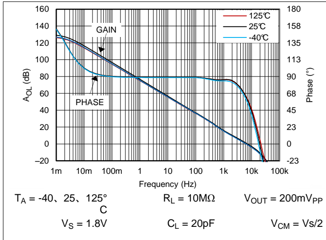
Figure 31. 开环增益和相位, 1.8V, 10MΩ 负载
