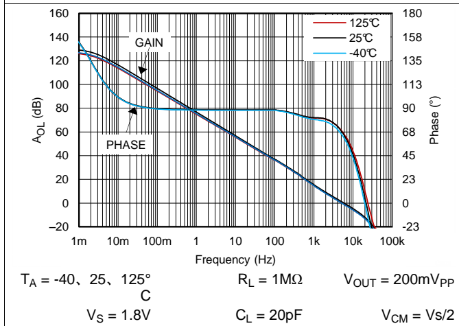
Figure 33. 开环增益和相位, 1.8V, 1MΩ 负载
