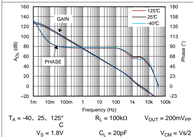
Figure 35. 开环增益和相位, 1.8V, 100kΩ 负载
