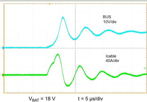
图 9-3. Disabled, 35-V, 1210, X7R C OUT Capacitor Without SMAJ18
