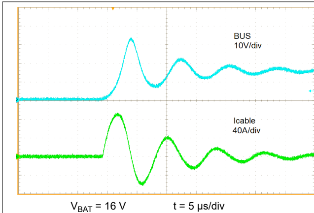
图 9-2. Disabled, 25-V, 1206, X7R C OUT Capacitor Without SMAJ16
