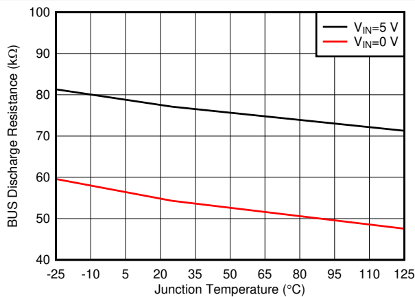
图 6-3. BUS Discharge Resistance (OVP) vs Temperature
