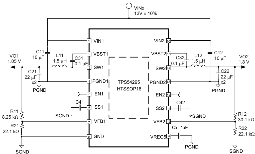
Figure 16. Schematic Diagram for the Design Example
