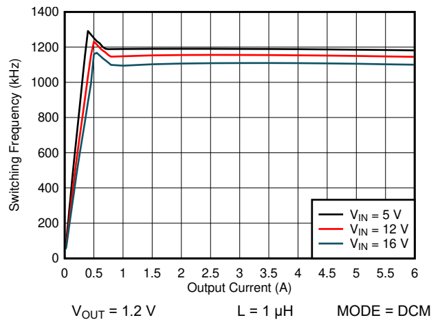
图 6-18. 1100-kHz Switching Frequency vs Load Current - DCM
