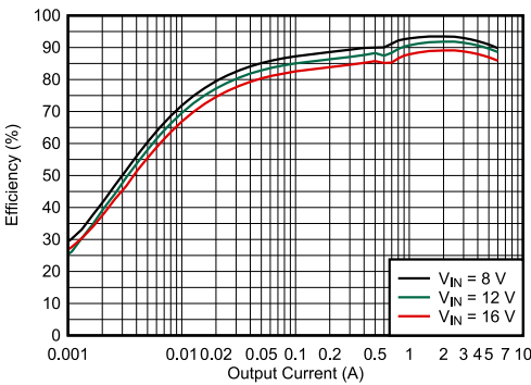
图 8-4. Efficiency - 1100 kHz, FCCM, External 3.3-V VCC, 4.7- \Omega R_{BOOT}
