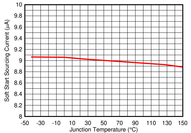
图 6-12. Soft-Start Sourcing Current
