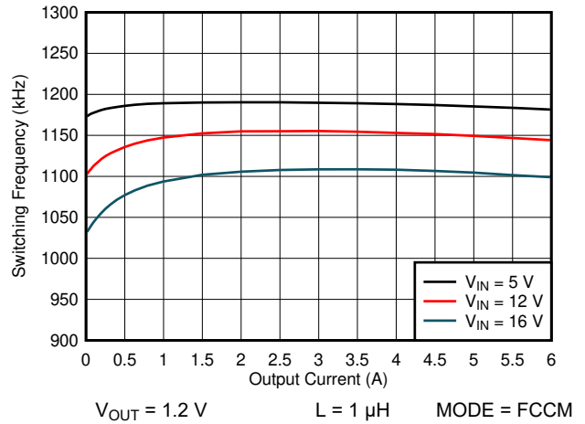
图 6-16. 1100-kHz Switching Frequency vs Load Current
