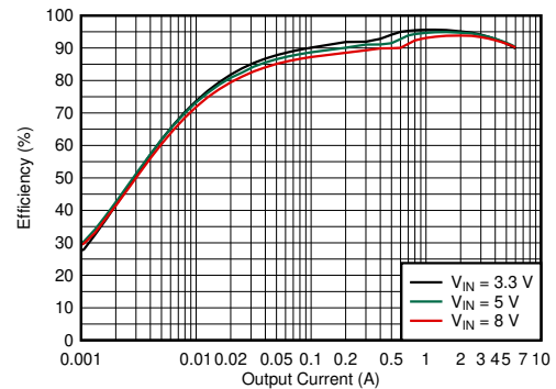
图 8-5. Efficiency - 1100 kHz, FCCM, External 3.3-V VCC, 0- \Omega R_{BOOT}
