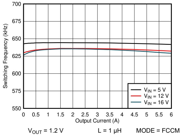
图 6-15. 600-kHz Switching Frequency vs Load Current
