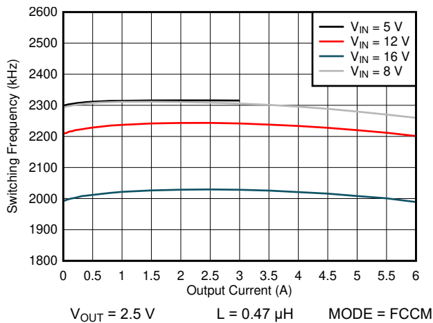
图 6-17. 2200-kHz Switching Frequency vs Load Current
