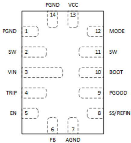
图 5-1. 14-Pin QFN RPG Package (Top View)
