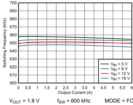
图 8-14. Switching Frequency vs Output Current - 600 kHz
