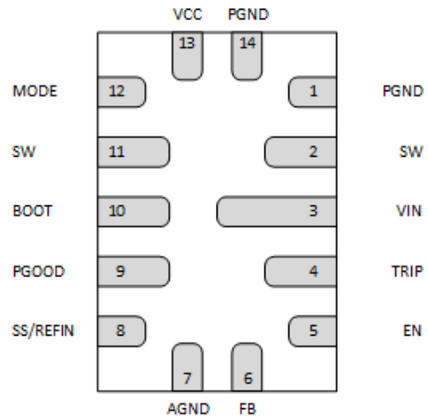
图 5-2. 14-Pin QFN RPG Package (Bottom View)
