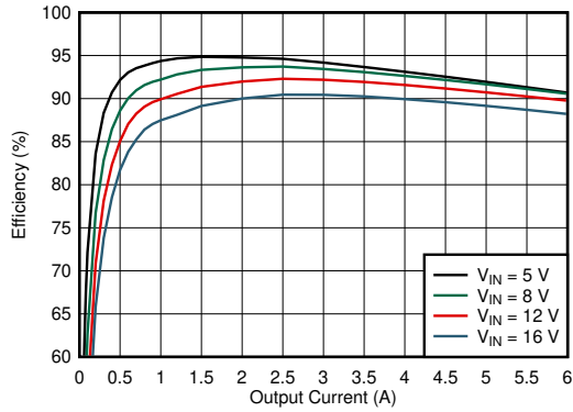
图 8-8. Efficiency - 600 kHz, FCCM
