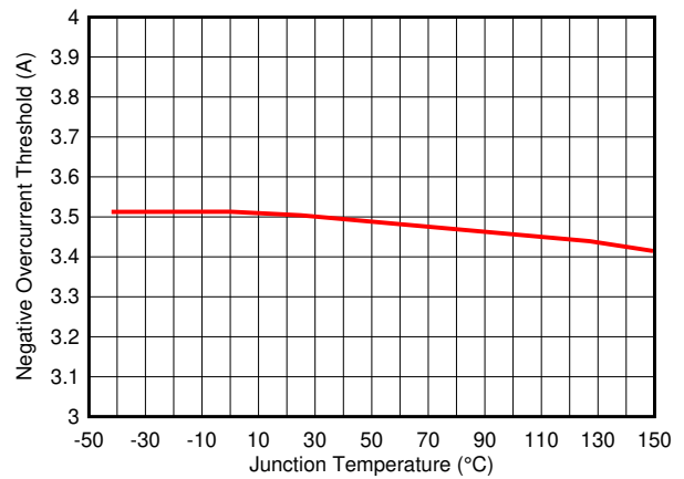
图 6-4. Negative Overcurrent Limit
