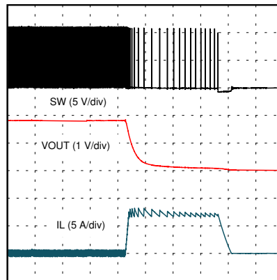
图 8-30. Short Circuit Response
