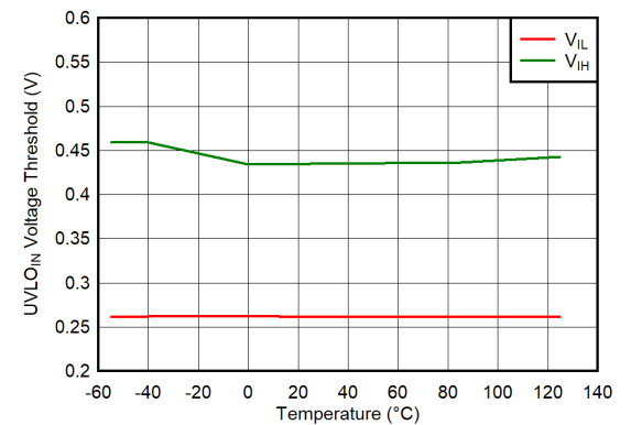
C_{IN} = C_{OUT} = 10\ \mu\text{F} , C_{BIAS} = 1\ \mu\text{F} , C_{SS} = 0\ \text{nF} , V_{BIAS} = 5\text{ V} , 1.1\text{ V} \leq V_{EN} \leq 6\text{ V}
