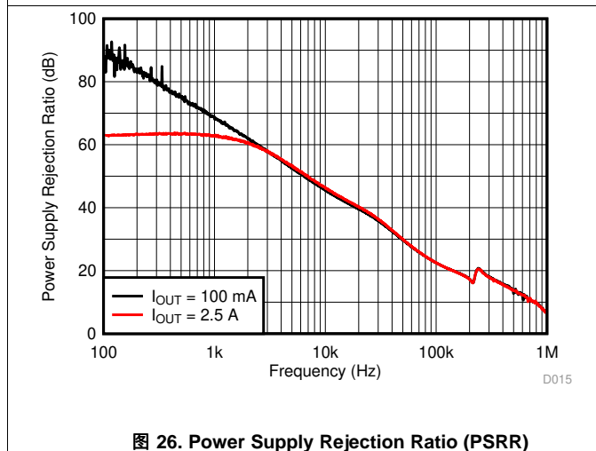
图 26. Power Supply Rejection Ratio (PSRR)
